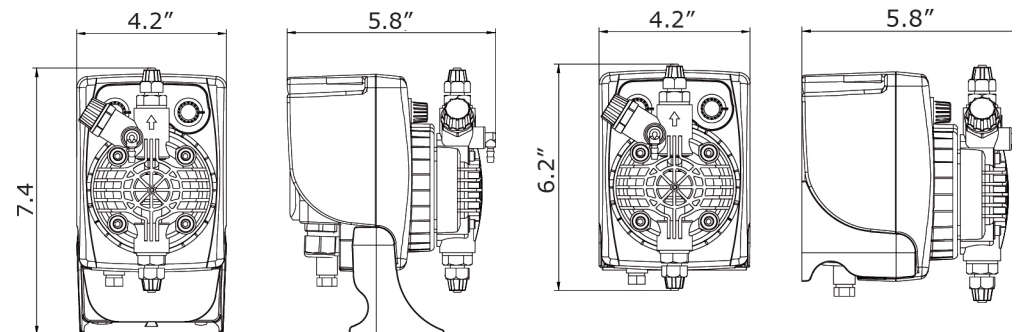
BASE MOUNT
