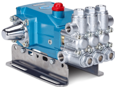
5CP6190 DIRECT DRIVE CAT PUMPS CERAMIC PLUNGER PUMPS
