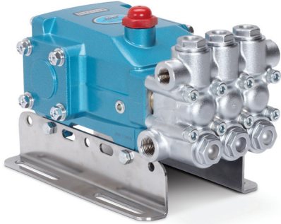
5CP2140WCS3 DIRECT DRIVE CAT PUMPS CERAMIC PLUNGER PUMPS
