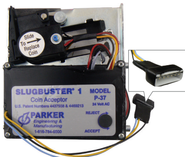
SLUGBUSTER (ACW4-5) HAMILTON CHANGER PARTS
