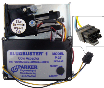
SLUGBUSTER (GOLD LINE) HAMILTON CHANGER PARTS
