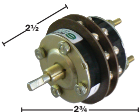
12 POSITION ROTARY SWITCH ELECTROSWITCH
