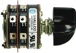
8 POSITION 2 STACK ROTARY SWITCH SHALLCO SWITCHES
