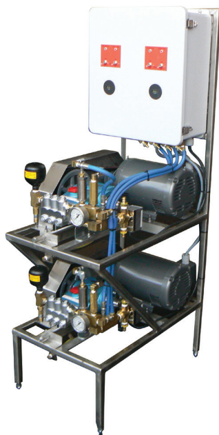
PUMP STAND
