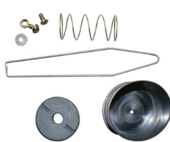
MAGNET KIT - OLD STYLE HYDROMINDER REPAIR PARTS
