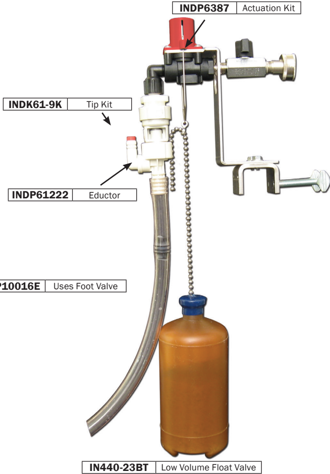
IN440-23BT Low Volume Float Valve
