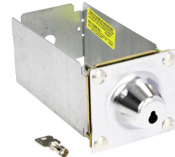
SPECIAL ULTRA GUARD MONEY BOX 5 5 / 8 " L x 3 3 / 4 " W x 2 1 / 2 " H GREENWALD
