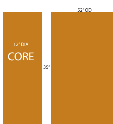
SIDE WASHER BRUSH 12 x 35 x 52 STRAIGHT CUT FIVE STAR CAR WASH FOR HANNA
