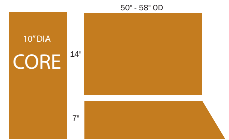
HUBCAP ROCKER PANEL 10 x 21 x 50/58 ANGLE CUT FIVE STAR CAR WASH FOR HANNA
