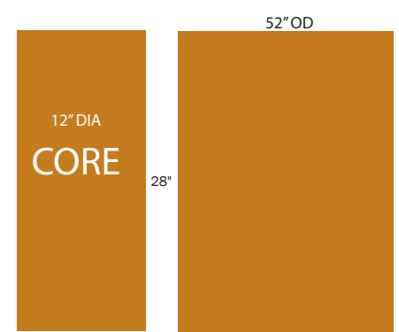
ROCKER PANEL SIDE WASHER 12 x 28 x 52 STRAIGHT CUT FIVE STAR CAR WASH FOR HANNA
