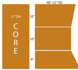
MODEL 2001 & 2x2 PASSENGER SIDE 28" HIGH CORE FIVE STAR CAR WASH FOR BELANGER
