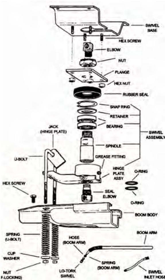
COMPLETE BOOM ASSEMBLY ZIERDEN COMPANY
