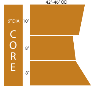
MODEL 2x2 DRIVER SIDE 26" HIGH CORE FIVE STAR CAR WASH FOR BELANGER
