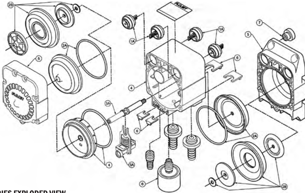
MODEL G57 SERIES EXPLODED VIEW FLOJET PUMPS
