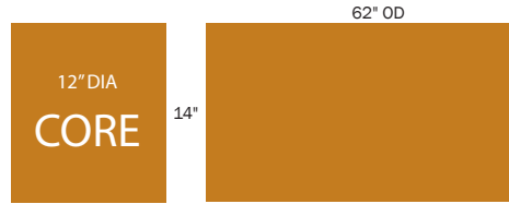
HORIZONTAL WINDOW WASHER 12 X 14 X 62 STRAIGHT CUT FIVE STAR CAR WASH FOR HANNA
