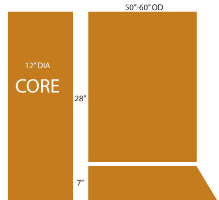
SIDE WASHER BRUSH 12 x 35 x 60 ANGLE CUT FIVE STAR CAR WASH FOR HANNA
